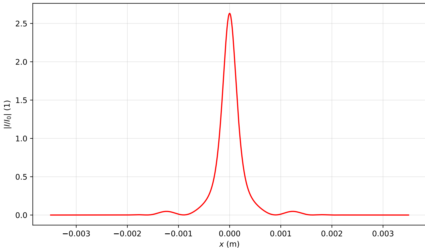
Intensity profile I(x, y = 0, z = 2.149)/I_0 , \text{Pin}=2.0\text{Pcr} , artificial time
